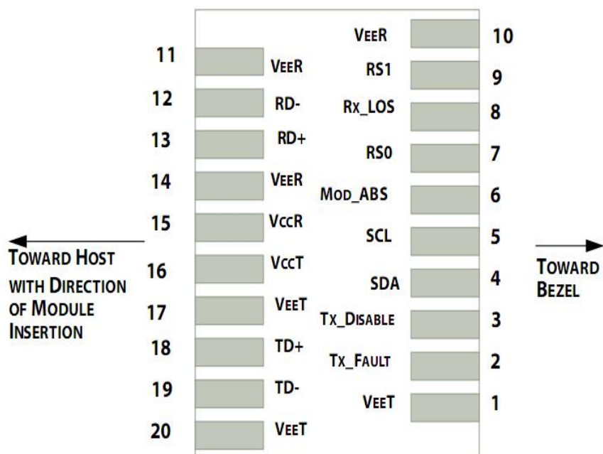
Pinout of Connector Block on Host Board
