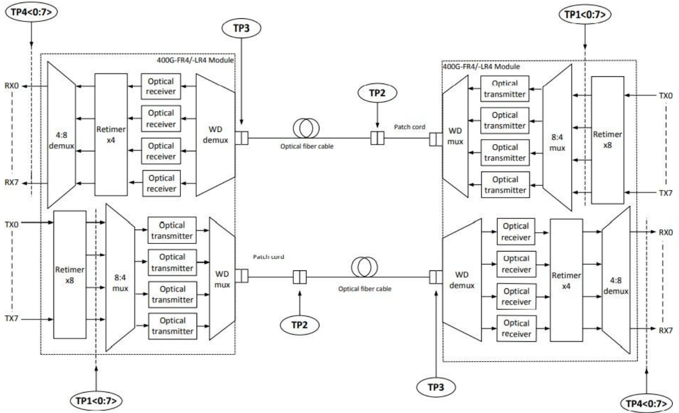
Figure 2. Module Block Diagram
