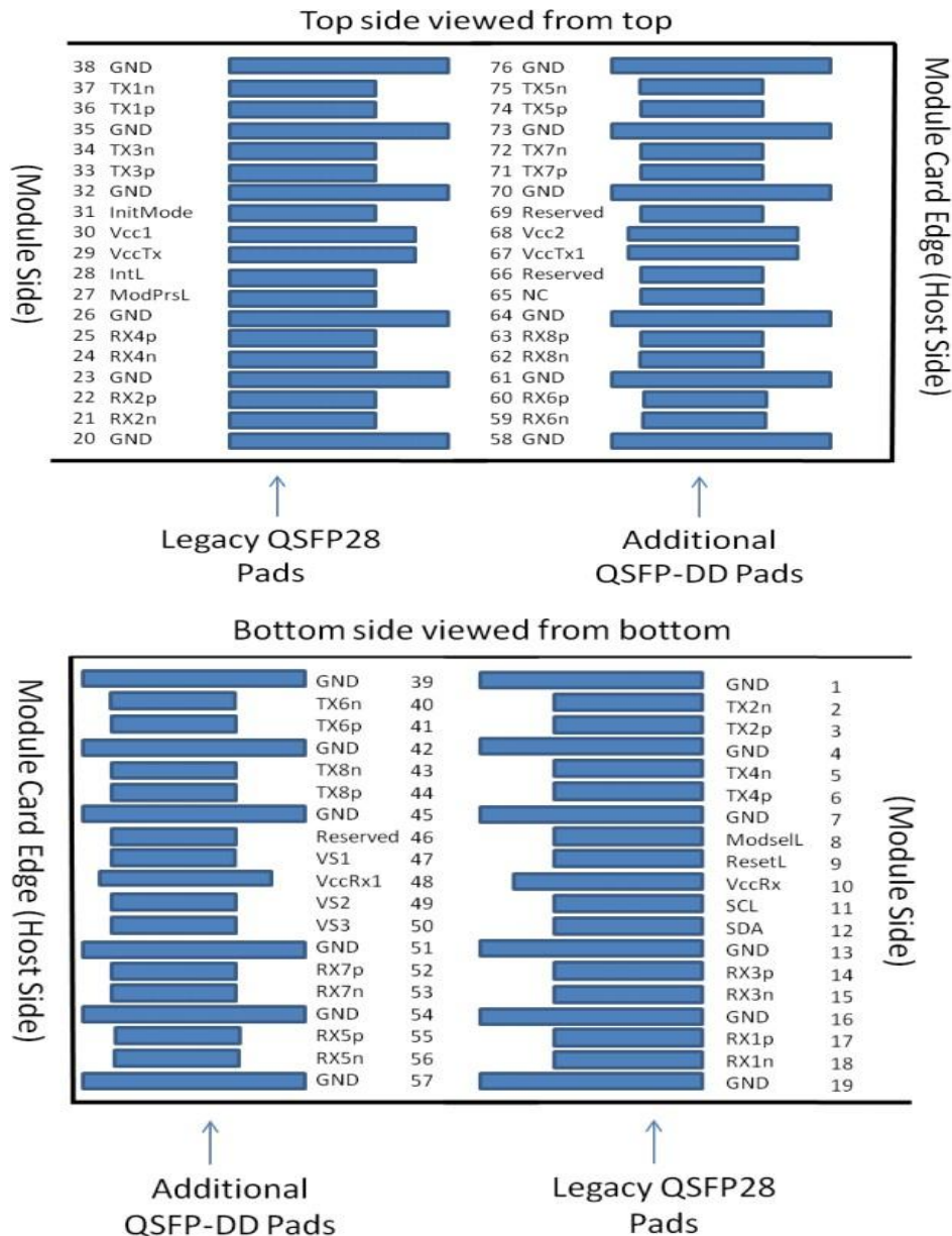
Figure 1. QSFP-DD pad assignment top view
