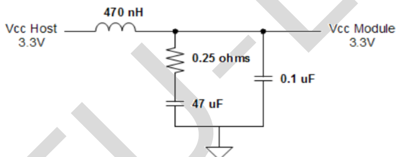
Figure 13-6: Host board power filter circuit
