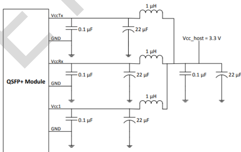
FIGURE 5-4 RECOMMENDED HOST BOARD POWER SUPPLY FILTERING
