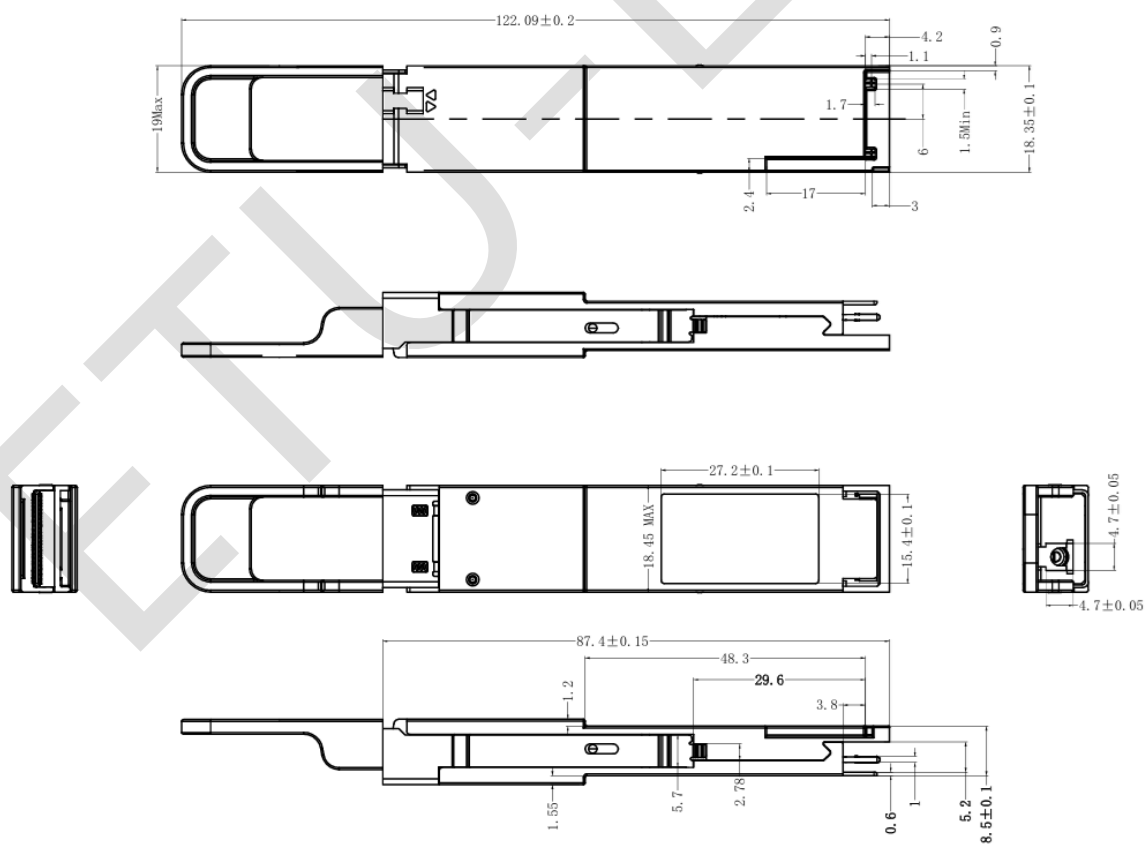
Mechanical Dimensions
