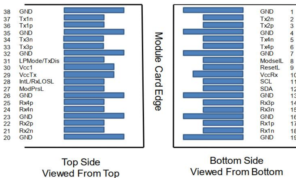
Figure 1. QSFP28-compliant 38-pin connector
