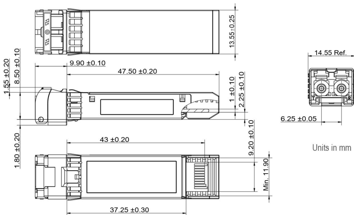
Figure2. Mechanical Outline
